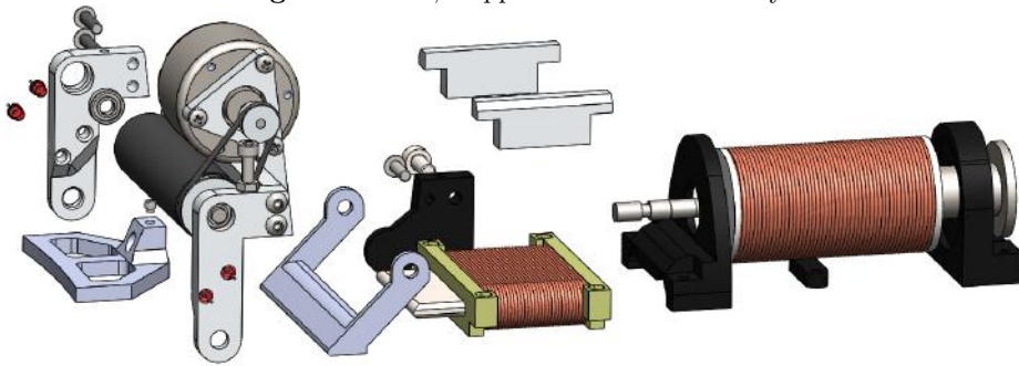
Fig. 4. Exploded view.
